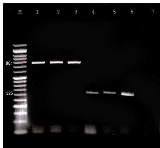
Fig. 3: Agarose gel electrophoresis of multiplex PCR-amplified products of SCCmec typing of MRSA. Lane M; DNA ladder (50 bp DNA Marker). Lanes 1-3; SCC type IVd (881 bp), Lanes 4-6; SCC type V (325 bp), lane 7; negative control.
