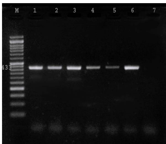
Fig. 2 : Agarose gel electrophoresis of PCR-amplified products of the Panton-valentine gene. Lane M; DNA ladder (50 bp DNA Marker). Lanes 1-6; PVL positive MRSA strains (433 bp). lane 7; negative control
