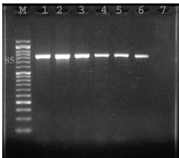
Fig. 1: Agarose gel electrophoresis of PCR-amplified products of the mecA gene. Lane M; DNA ladder (50 bp DNA Marker). Lanes 1-6; MRSA (851 bp). Lane 7; negative control
